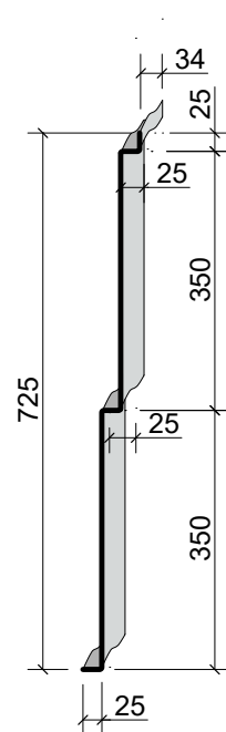
B-B Section
