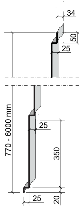
B-B Section
