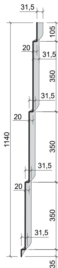
B-B Section
