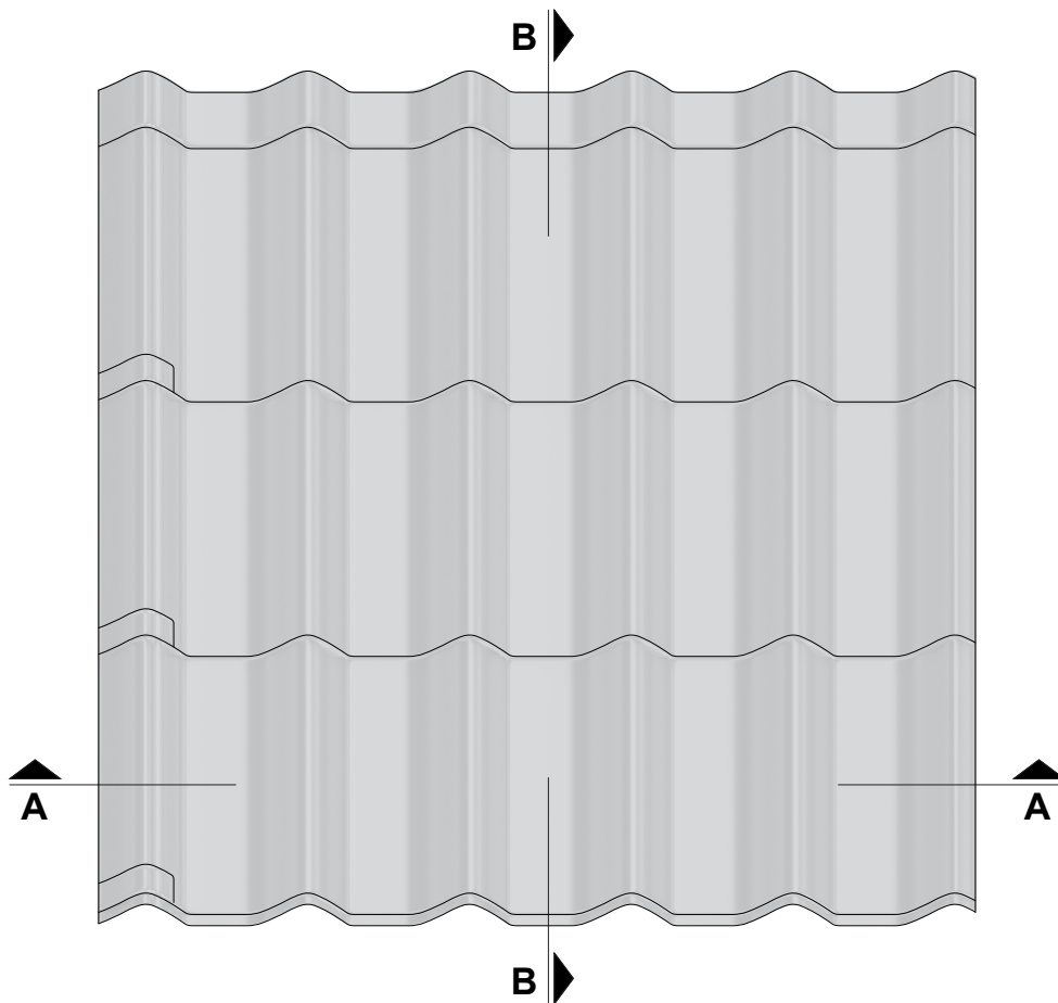
Plan view
