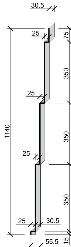
B-B Section
