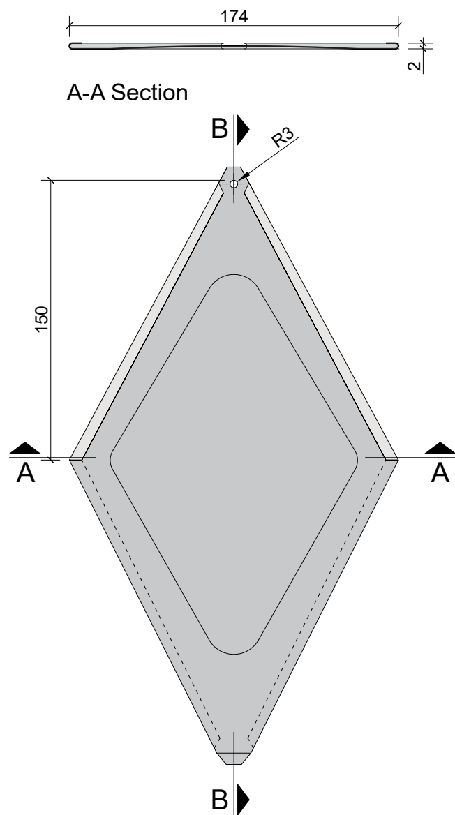
Plan view
